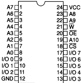
Pinout DIL 24 pins (top view)
