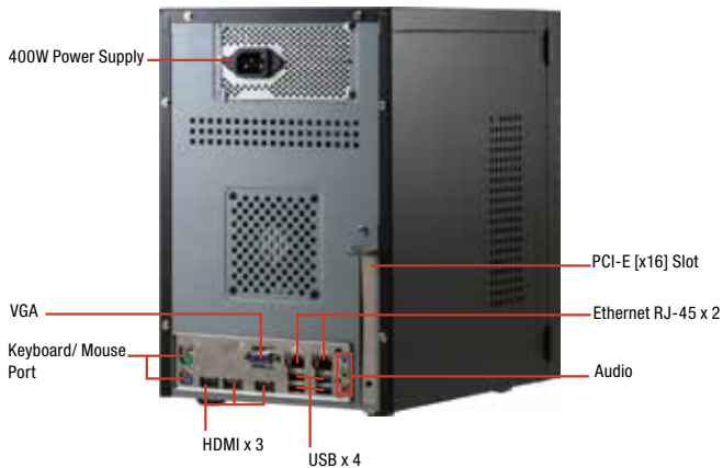
Rear View
