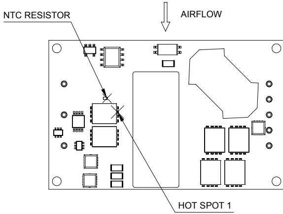
Figure 19: Temperature measurement location.* The allowed maximum hot spot1 temperature is defined at 125
