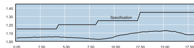
Typical SWR of a Model 4T-10
