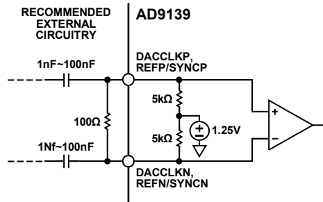
Figure 42. Clock Receiver Input Simplified Equivalent Circuit
