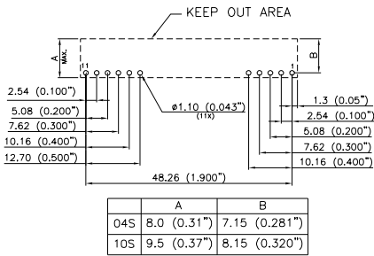
RECOMMENDED P.W.B PAD LAYOUT
