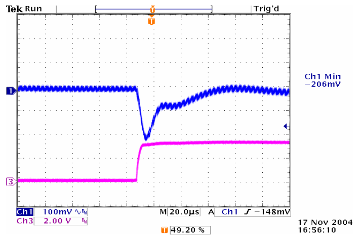
Figure 20: Typical transient response to step load change at 2.5A/\mu S from 50% to 100% of I_o , max at 5Vin, 3.3V out (Cout = ceramic, 10μF tantalum)
