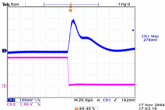
Figure 23: Typical transient response to step load change at 2.5\text{A}/\mu\text{S} from 100% to 50% of I_o , max at 3.3\text{V}_{in} , 2.5\text{V}_{out} ( C_{out} = ceramic, 10\mu\text{F} tantalum)
