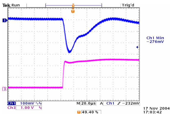
Figure 24: Typical transient response to step load change at 2.5\text{A}/\mu\text{S} from 50% to 100% of I_o , max at 3.3\text{V}_{in} , 2.5\text{V}_{out} ( C_{out} = ceramic, 10\mu\text{F} tantalum)
