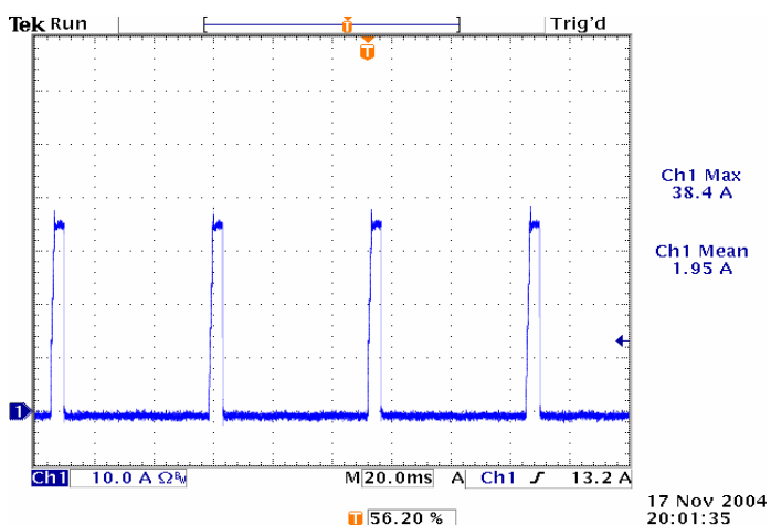
Figure 27: Output short circuit current 5\text{V}_{in} , 0.75\text{V}_{out}
