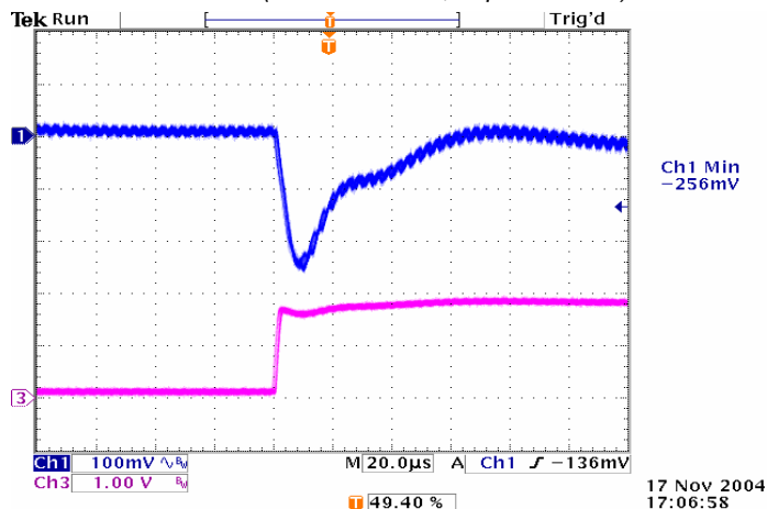
Figure 26: Typical transient response to step load change at 2.5\text{A}/\mu\text{S} from 50% to 100% of I_o , max at 3.3\text{V}_{in} , 1.8\text{V}_{out} ( C_{out} = ceramic, 10\mu\text{F} tantalum)
