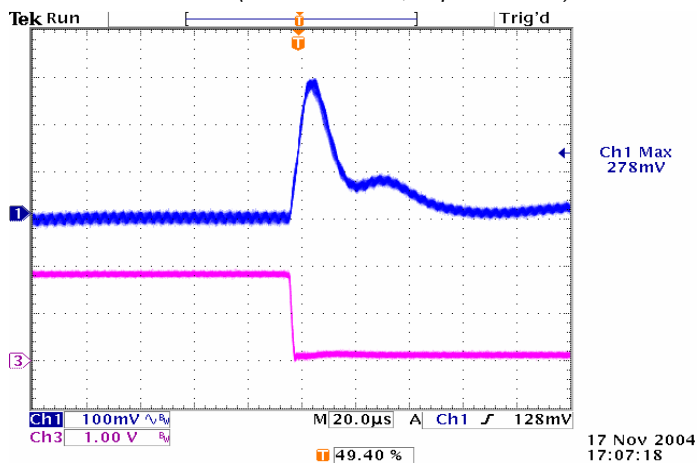
Figure 25: Typical transient response to step load change at 2.5\text{A}/\mu\text{S} from 100% to 50% of I_o , max at 3.3\text{V}_{in} , 1.8\text{V}_{out} ( C_{out} = ceramic, 10\mu\text{F} tantalum)
