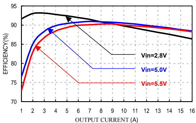
Figure 3: Converter efficiency vs. output current (1.8V out)
