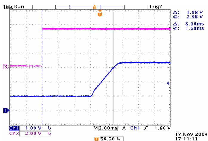
Figure 28: Turn on with Prebias 5\text{V}_{in} , 3.3\text{V}/0\text{A}_{out} , V_{bias}=1.0\text{V}_{dc}
