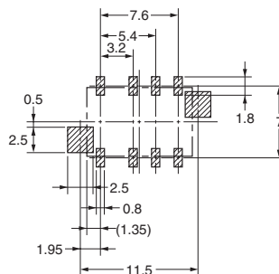
Mounting Dimensions (Top View) Tolerance: \pm 0.1 mm
