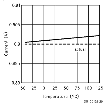
Accuracy vs Temperature (LM3812-1.0 and LM3813-1.0)
