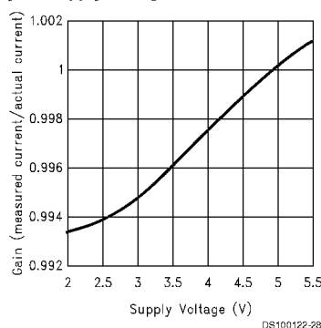
Accuracy vs Supply Voltage
