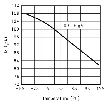
Operating Current vs Temperature
