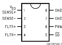
Top View LM3812
