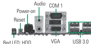
Red LED: HDD Green LED: power-on ▲ AX93275
