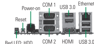
Red LED: HDD Green LED: power-on ▲ AX93276
