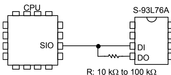
Figure 14 Connection of 3-Wire Interface
