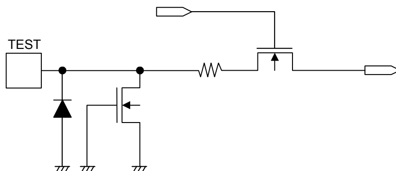
Figure 17 TEST Pin
