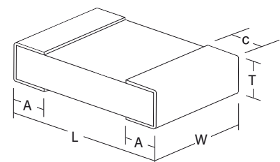
Wrap-around terminations (3 faces)
