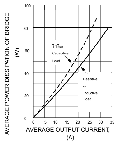
FIG.6-MAXIMUM POWER DISSIPATION
