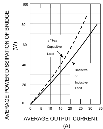
FIG.6-MAXIMUM POWER DISSIPATION
