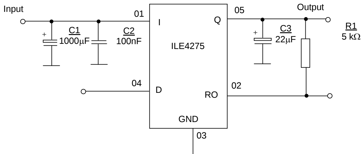
Typical Application Diagram
