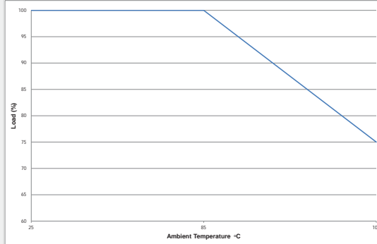
NCS1S2403SC
