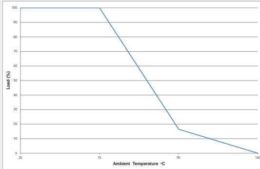
NCS1S1212SC
