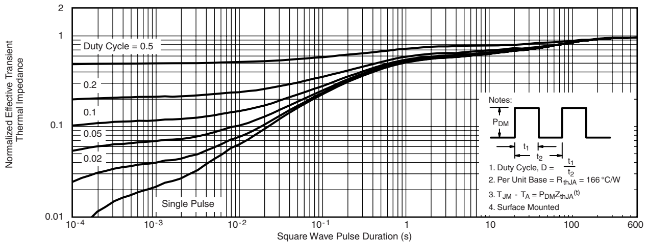
Normalized Thermal Impedance, Junction-to-Ambient
