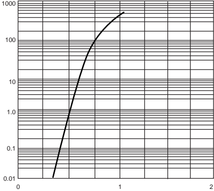
FIG. 1- FORWARD CHARACTERISTICS
