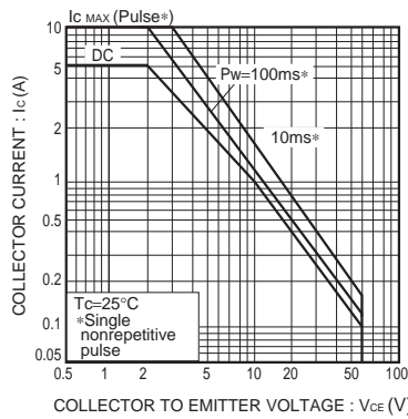
Fig.8 Safe operating area
