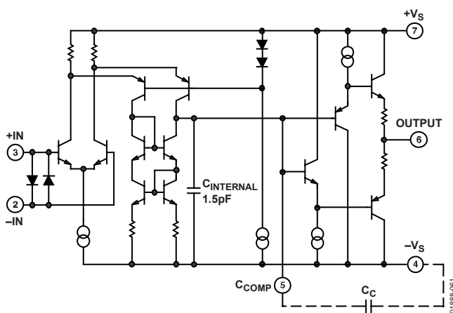
Figure 61. Simplified Schematic
