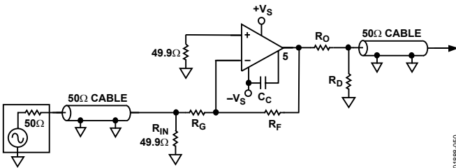
Figure 50. Inverting Gain
