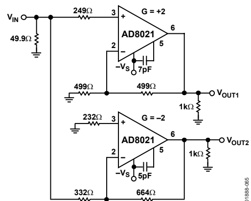
Figure 65. Differential Amplifier
