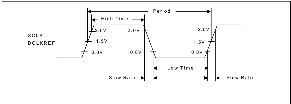
Figure 3. 3.3V Clock Duty Cycle
