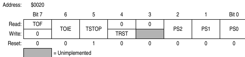
Figure 11-5. TIM Status and Control Register
