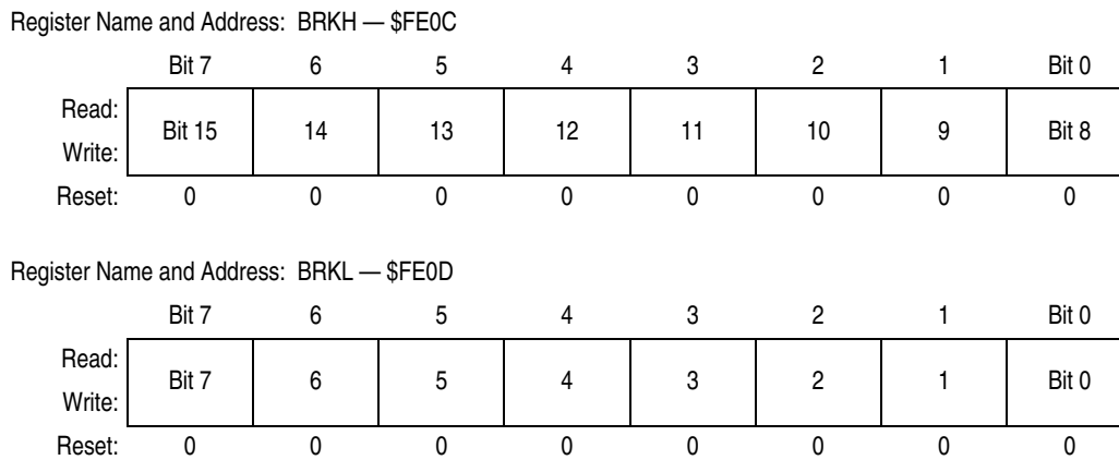
Figure 13-4. Break Address Registers (BRKH and BRKL)
