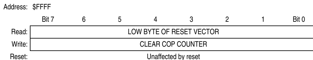
Figure 4-2. COP Control Register (COPCTL)
