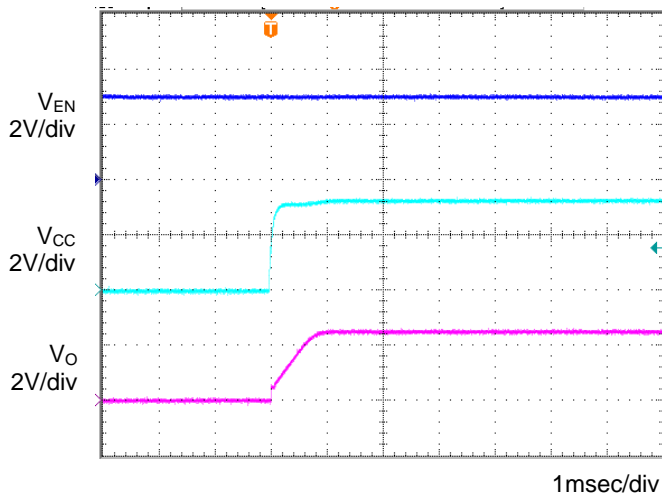
Figure 9. Input sequence 1 Co=1µF, Ta=-40°C
