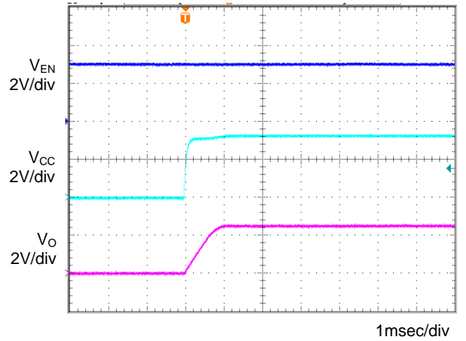
Figure 10. Input sequence 1 Co=1µF, Ta=25°C
