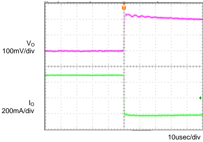
Figure 7. Transient Response (0.5→0A) Co=1µF, Ta=25°C
