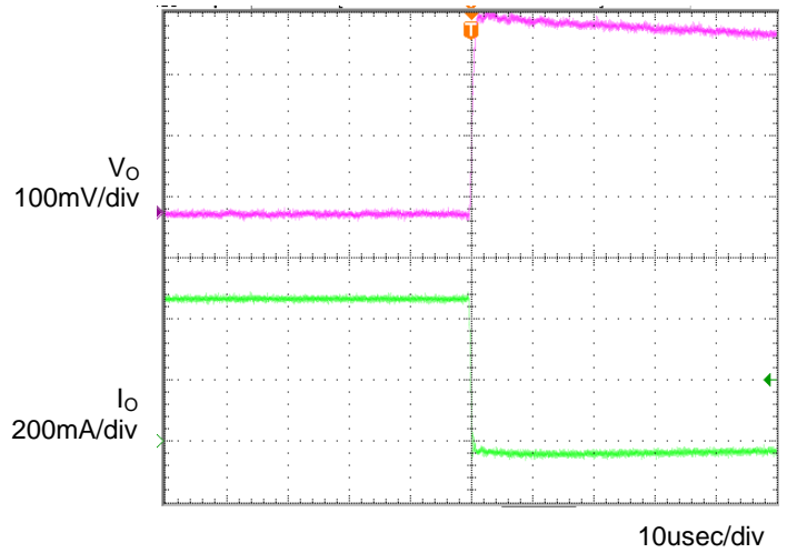
Figure 8. Transient Response (0.5→0A) Co=1µF, Ta=105°C
