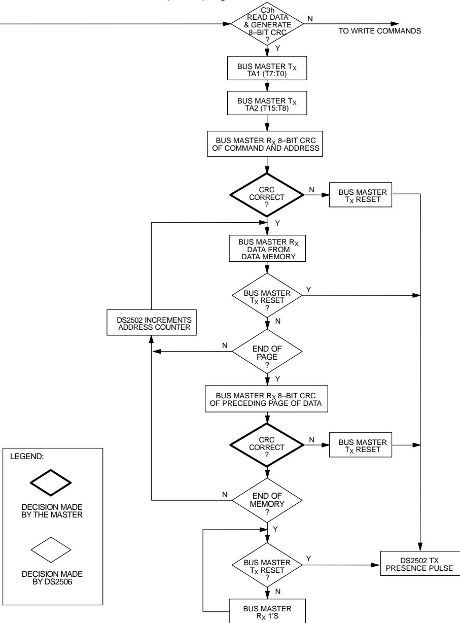
MEMORY FUNCTION FLOW CHART (cont'd) Figure 6
