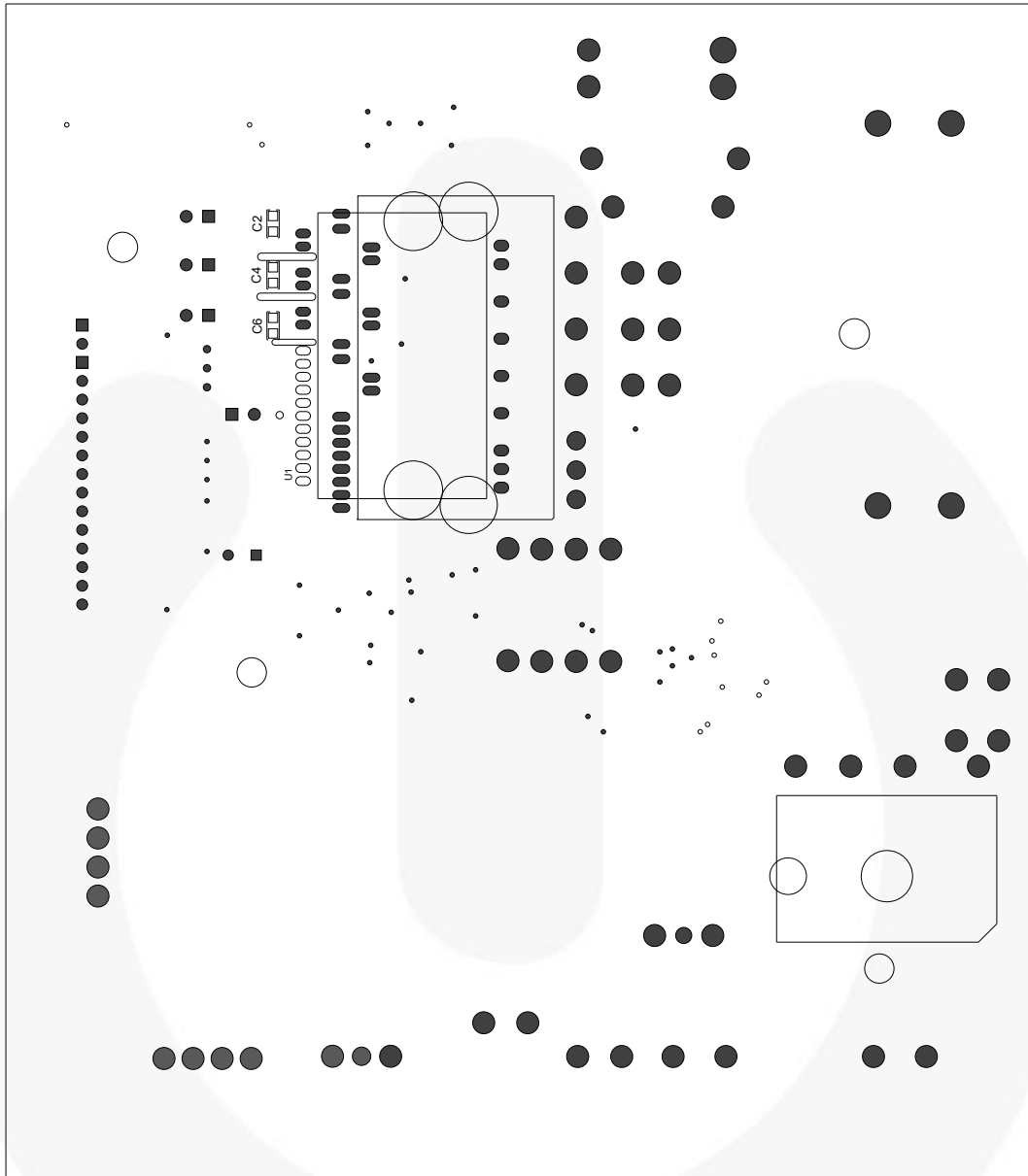
Figure 18. Bottom Assembly
