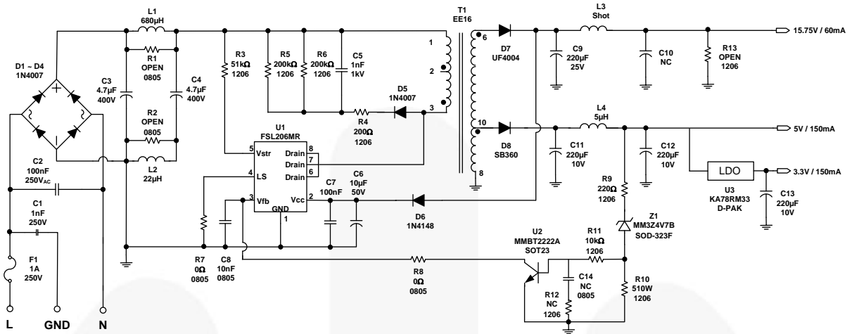
Figure 14. PS1 Schematic
