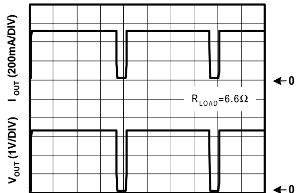
Overtemperature Shutdown
