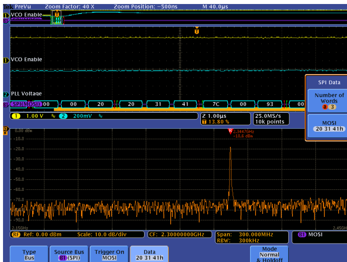
Capture - Triggering on a specific transmit data packet going across a SPI bus. A complete set of triggers, including triggers for specific serial packet content, ensures you quickly capture your event of interest.
