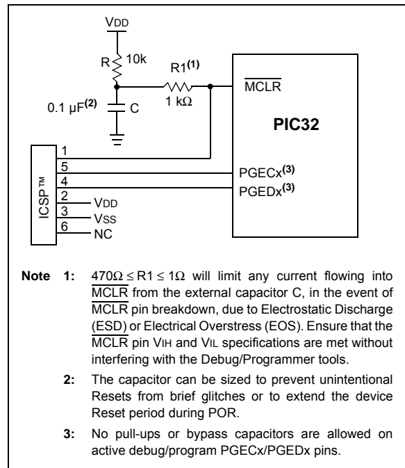
FIGURE 2-2: \overline{\text{MCLR}} PIN CONNECTIONS
