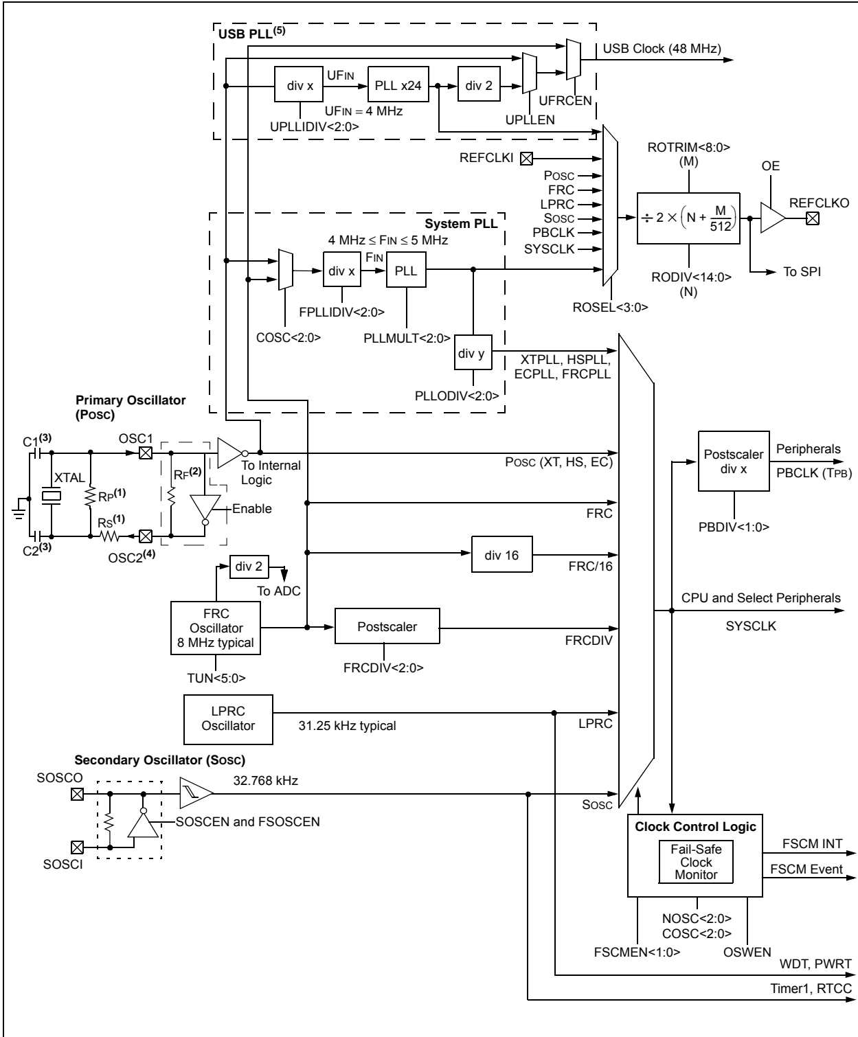
FIGURE 8-1: OSCILLATOR DIAGRAM
