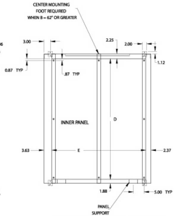
Rear View (Cross Section)
