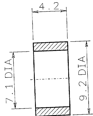
Retaining Ring
