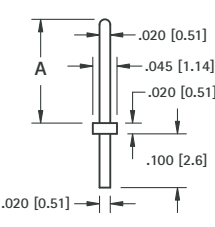
.020 (.51) PIN - SOLDER MOUNT
