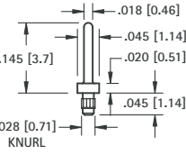
.018 (.46) PIN - PRESS-FIT
