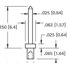
.025 (.64) PIN - SWAGE MOUNT
