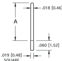
.018 (.46) PIN - PRESS-FIT
