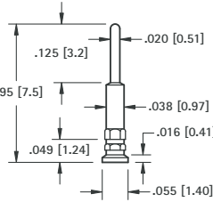
.020 (.51) PIN - PRESS-FIT
