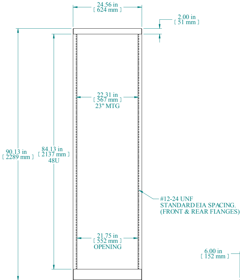
FRONT VIEW
