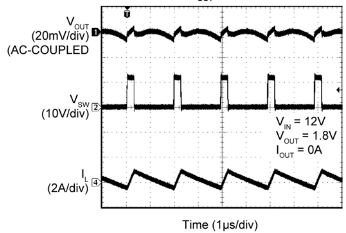
Switching Waveforms
