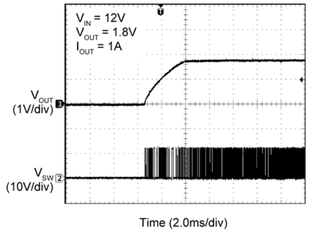
Output Recovery from Thermal Shutdown
