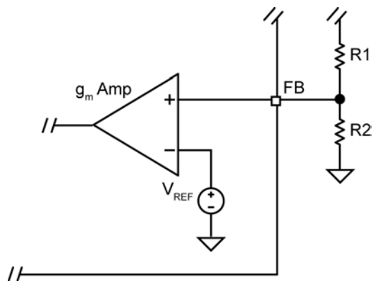
Figure 8. Voltage-Divider Configuration
