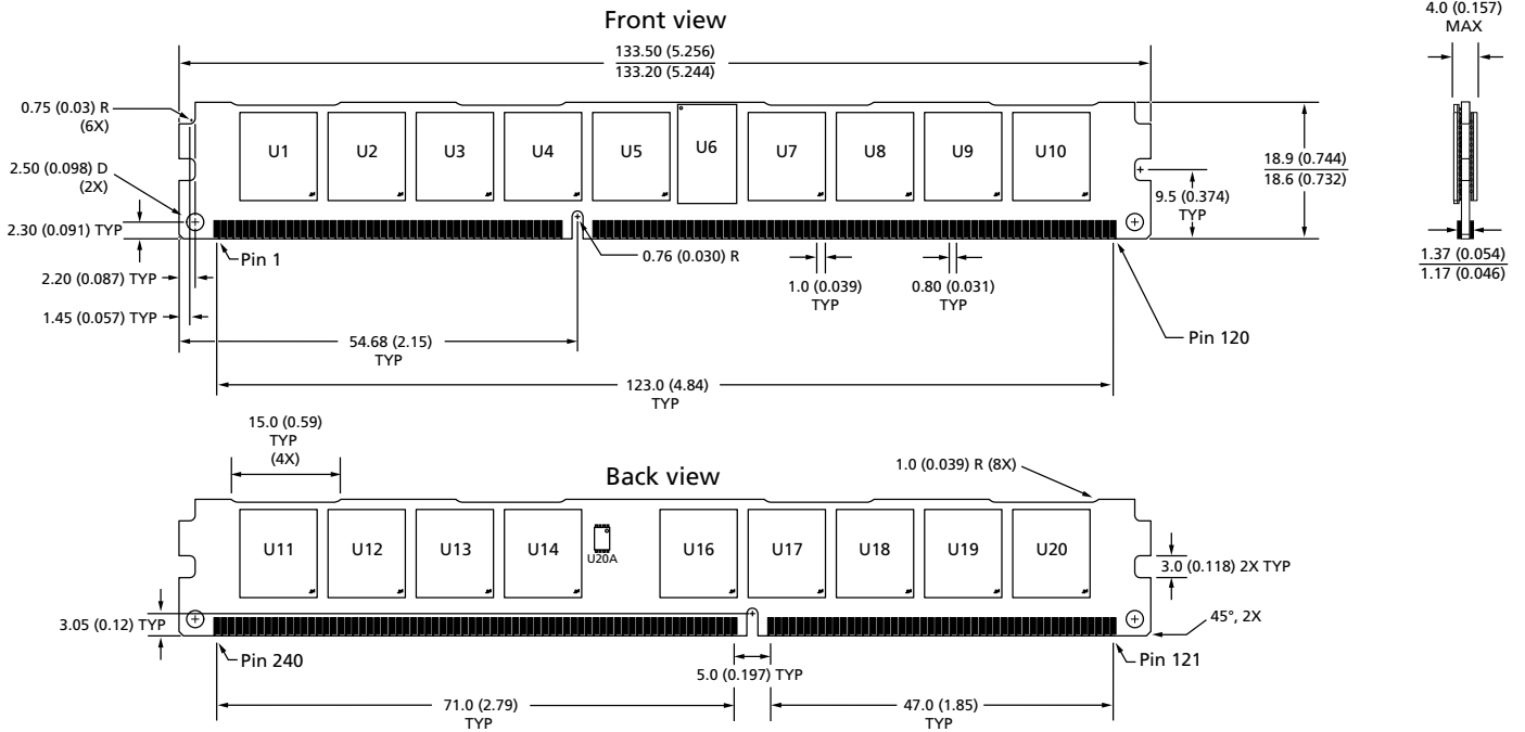
Figure 3: 240-Pin DDR3 VLP RDIMM
