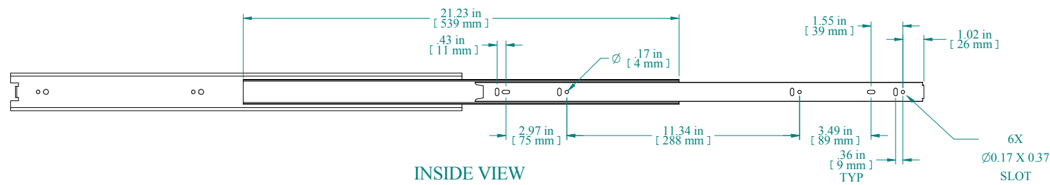
SLIDE RAIL MOUNT BRACKETS
