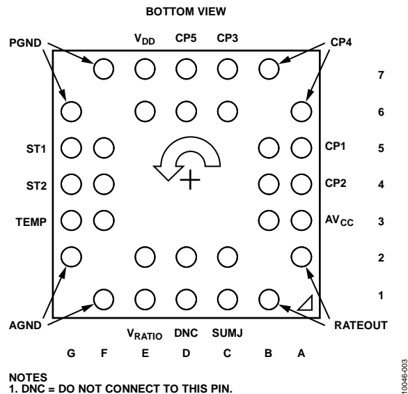
Figure 3. Pin Configuration
