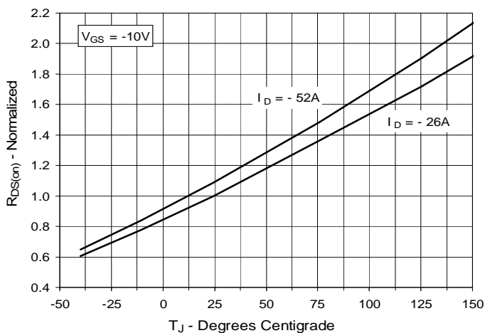
Fig. 4. R_{DS(on)} Normalized to I_D = -26\text{A} vs. Junction Temperature
