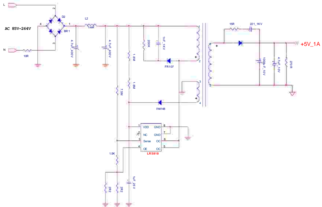
SOP-8 Application Circuit
