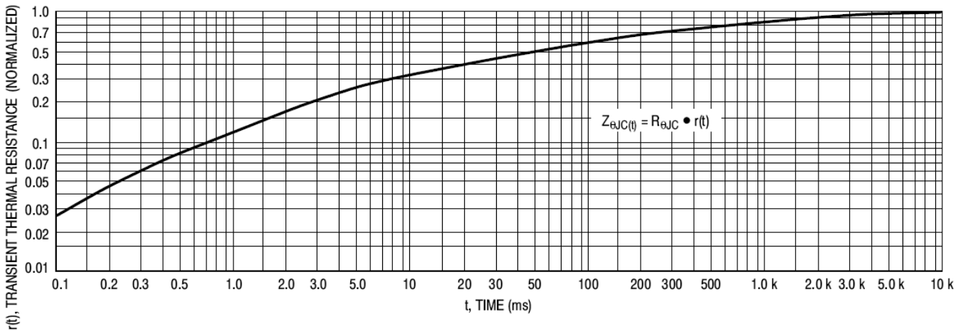
Figure 5. Thermal Response
