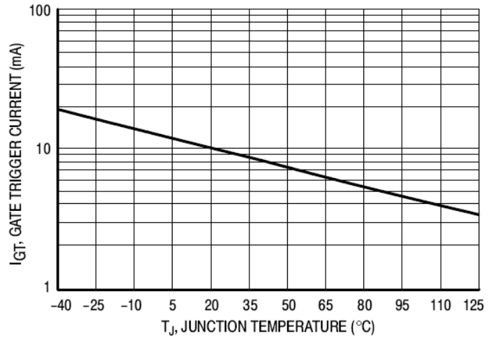
Figure 7. Typical Gate Trigger Current versus Junction Temperature
