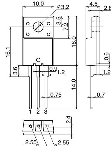
[TO-220FI(LS)]
