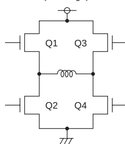
Single-phase motor (H-Bridge)
