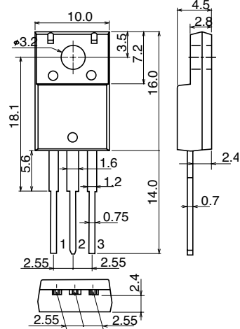
[TO-220ML]
