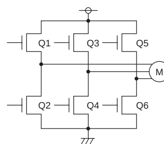
3-phase motor
