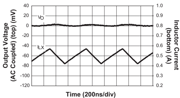
Output Ripple
