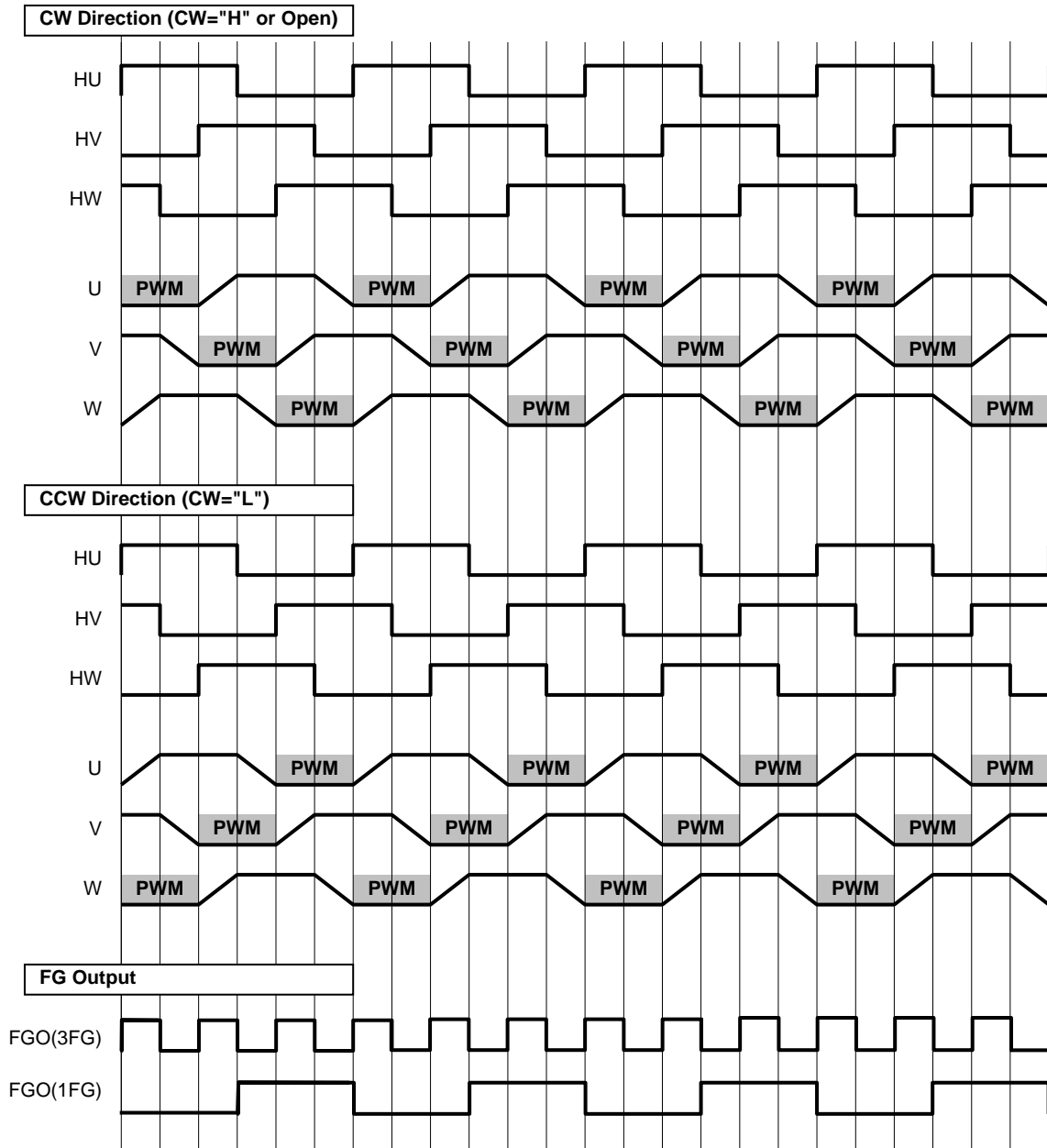
Figure 4. Timing Chart
