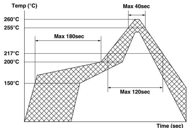
Figure 10.1 Recommended Reflow Solder Profile
