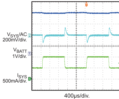
SYS Load Transient, Boost Mode
