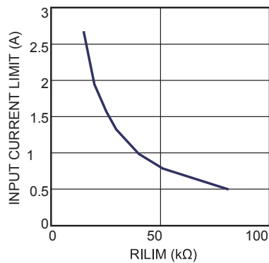
Input Current Limit Setting (I in_lim vs. R LIM )
