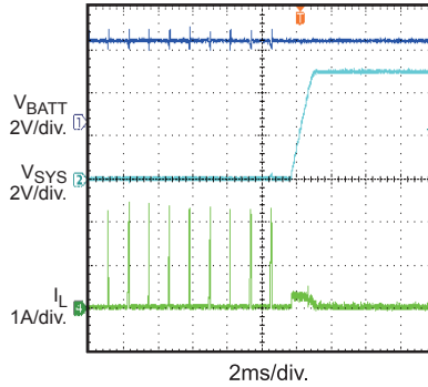
SYS Short Recovery Boost Mode
