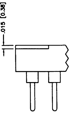
VIEW "A" SCALE 4:1
