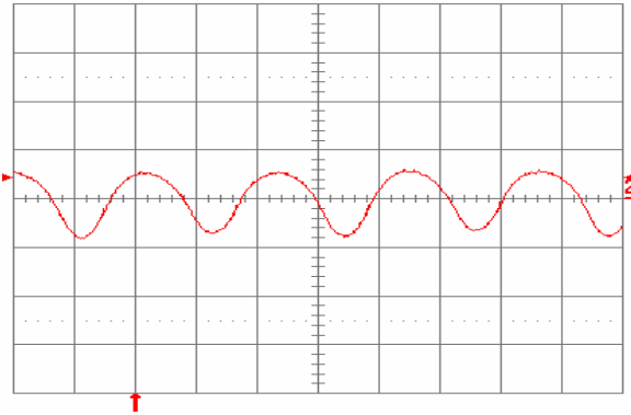
Fig. 1.5V.13: Input reflected ripple-current, i_c (100 mA/div.), measured at input terminals at full rated load current and V_{in} = 48 V. Refer to Fig. 1.5V.12 for test setup. Time scale: 1 \mu s/div.
