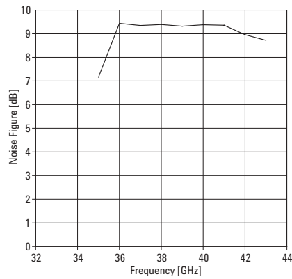
Figure 4. Typical Noise Figure
