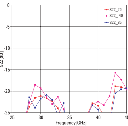
Figure 8. Typical S22 over temperature
