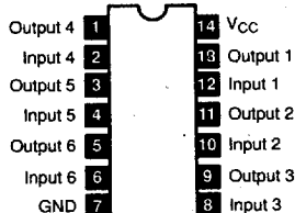
NTE74C901, NTE74C902, NTE74C903, NTE74C904 14-Lead DIP, See Diag. 247 Hex Buffer (CMOS)
