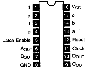
NTE74C925 16-Lead DIP, See Diag. 249 4-Digit Counter \bar{W} /Multiplexed Seven-Segment Output Driver
