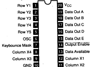
NTE74C923 20-Lead DIP, See Diag. 294 CMOS, 20-Key Keyboard Encoder \bar{W} /3-State Output
