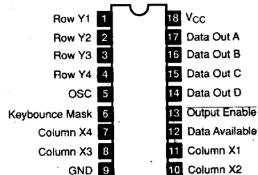
NTE74C922 18-Lead DIP, See Diag. 298 CMOS, 16-Key Keyboard Encoder \bar{W} /3-State Output
