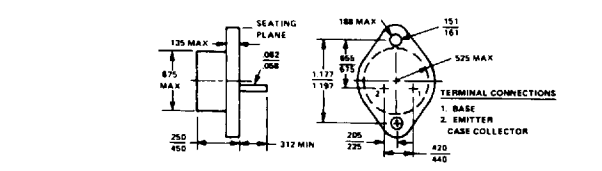
TO-3 (60 mil pins)
