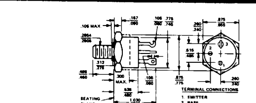
TO-63
