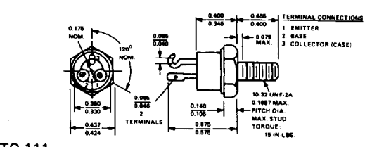
TO-111
