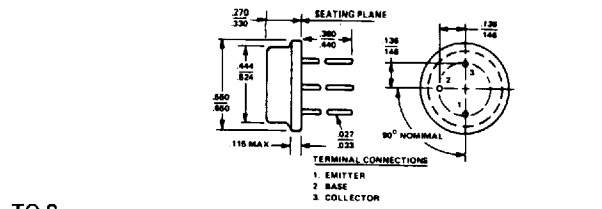
TO-8
