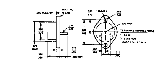
TO-66
