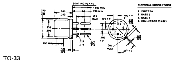
TO-33
