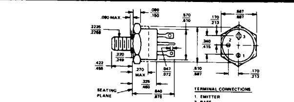
TO-61 (ISOLATED)
