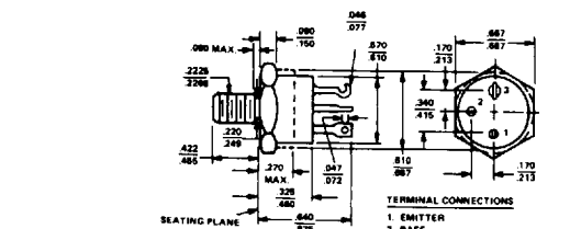
TO-61
