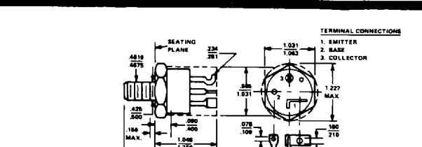
TO-114
