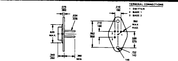
3 PIN TO-66
