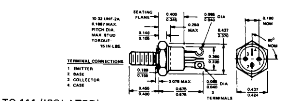
TO-111 (ISOLATED)
