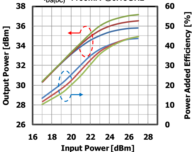
Input Power vs. Output Power, Power Added Efficiency by Drain Voltage I_{DS(DC)}=1100\text{mA} @6.15GHz
