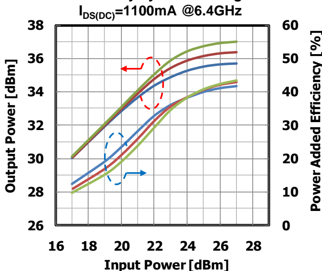
Input Power vs. Output Power, Power Added Efficiency by Drain Voltage I_{DS(DC)}=1100\text{mA} @6.4GHz
