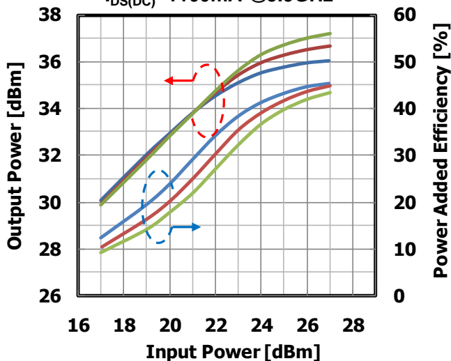
Input Power vs. Output Power, Power Added Efficiency by Drain Voltage I_{DS(DC)}=1100\text{mA} @5.9GHz
