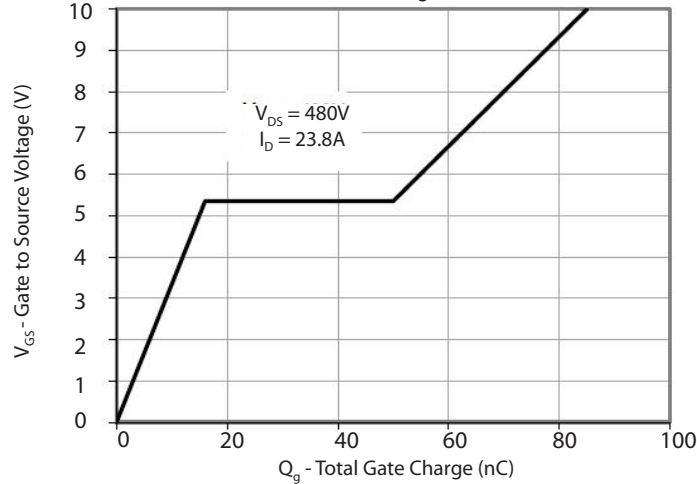
Gate Charge
